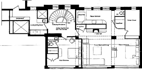
SECOND LEVEL FLOOR PLAN (w/ Proposed Bedroom Addition)
